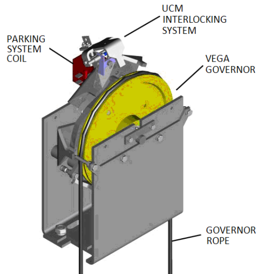
FIGURE 3: Vega Governor
