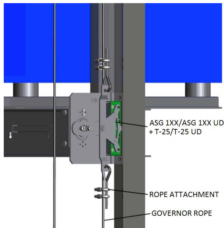
FIGURE 4: ASG 1 XX Safety Gear + T-25 Steering mechanism
